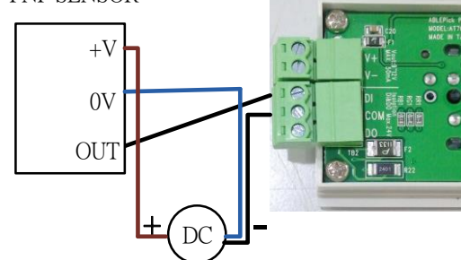
PNP SENSOR
