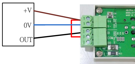
NPN SENSOR
