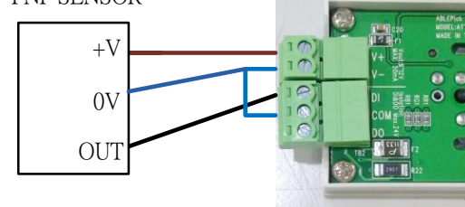
PNP SENSOR
