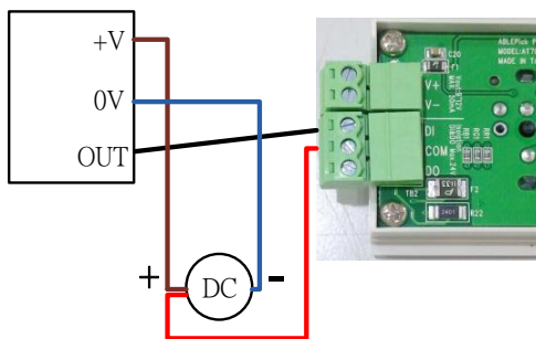
NPN SENSOR
